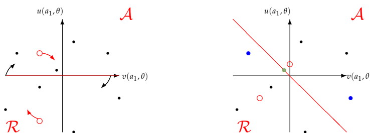
Figure 2: The optimal partition
